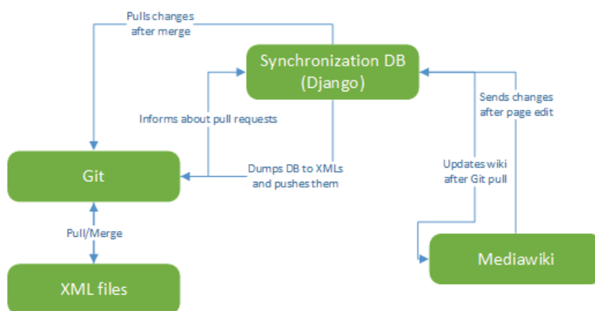
Figure 2: System architecture
