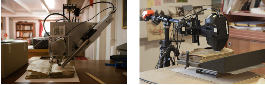
Fig. 5: The self-built XRF spectrometer with the Sinai Psalter in St. Catherine's Monastery (left) and the instrument ELIO (XGLab, Milano, Italy) measuring the Cod. Suprasliensis in the restoration department of the Slovenian State and University Library, Ljubljana (right).
